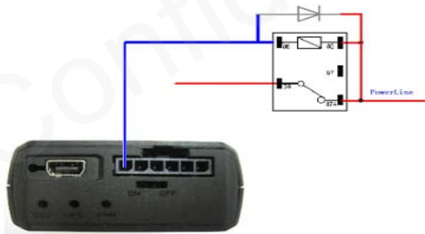
Figure 12. Typical Connection with Relay
